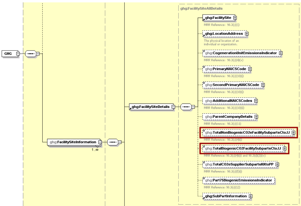
Figure 32 Facility-Level Roll-up Emissions Schema Diagram
